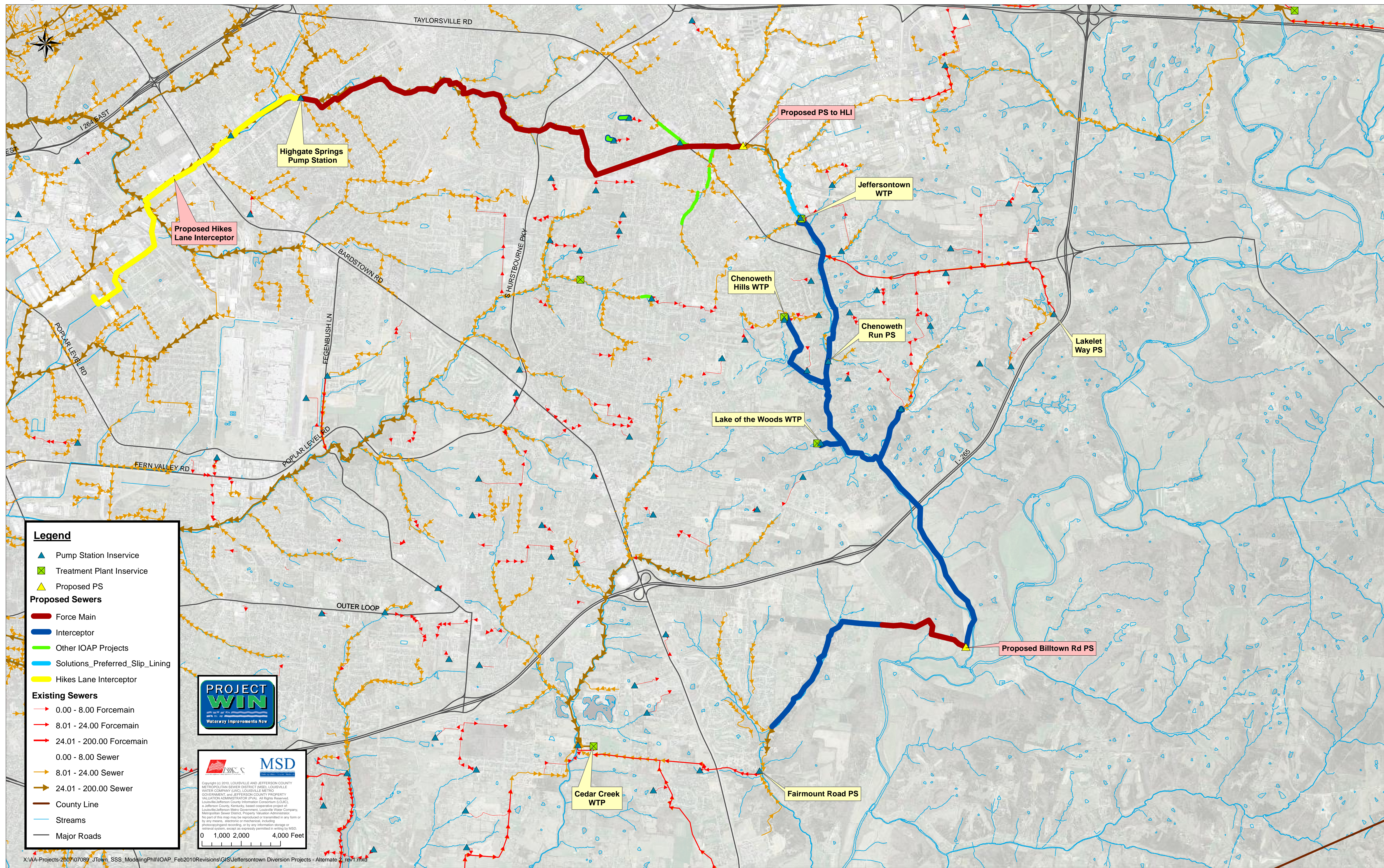
Figure 7 - Jeffersontown Diversion Projects: Alternate 2 - Grassland PS to HLI & Gravity and Pumped to Cedar Creek
