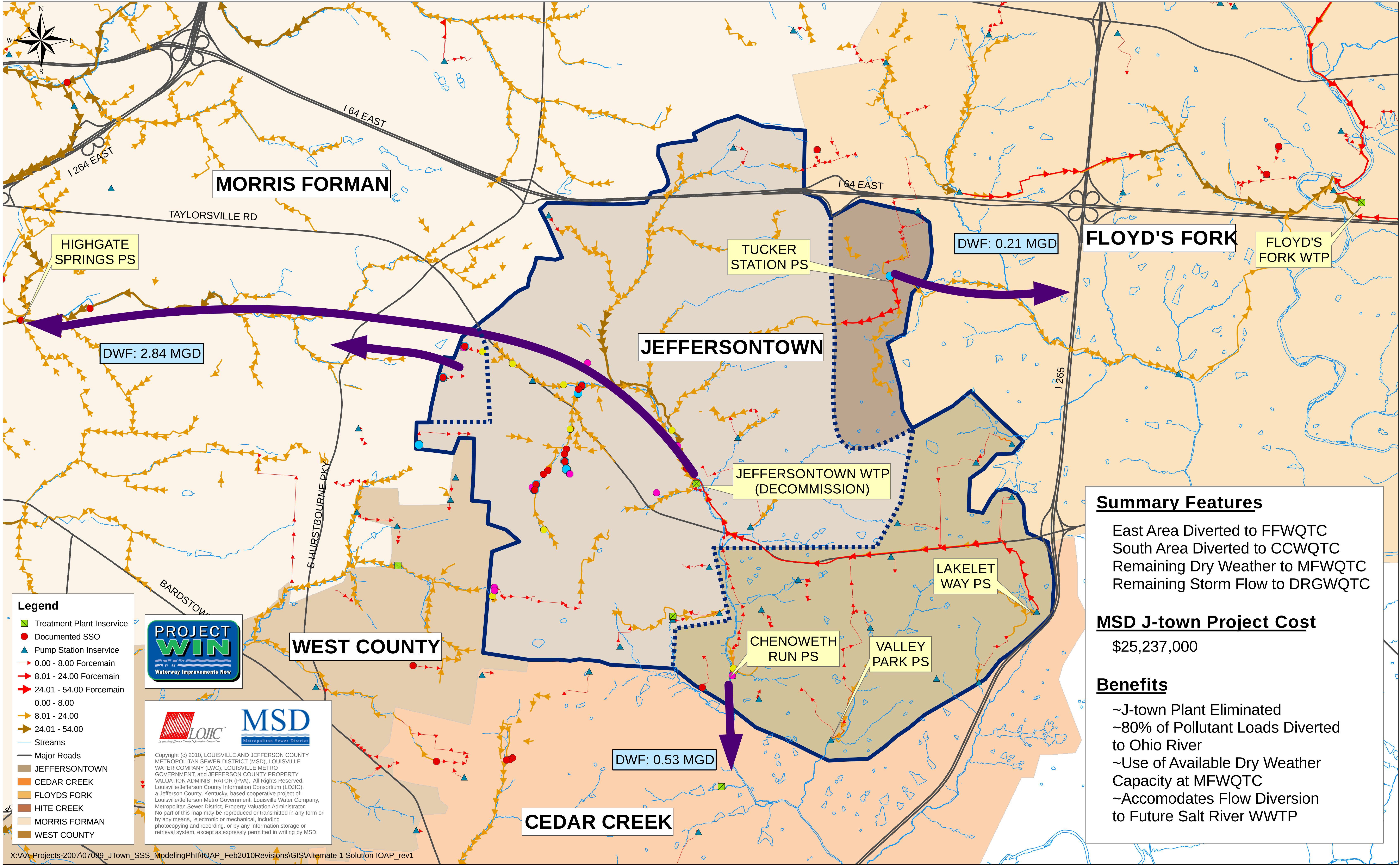
Figure 4 - Jeffersontown Diversion Projects: Alternate 1 - Gravity to HLI / Pumped to Cedar Creek
