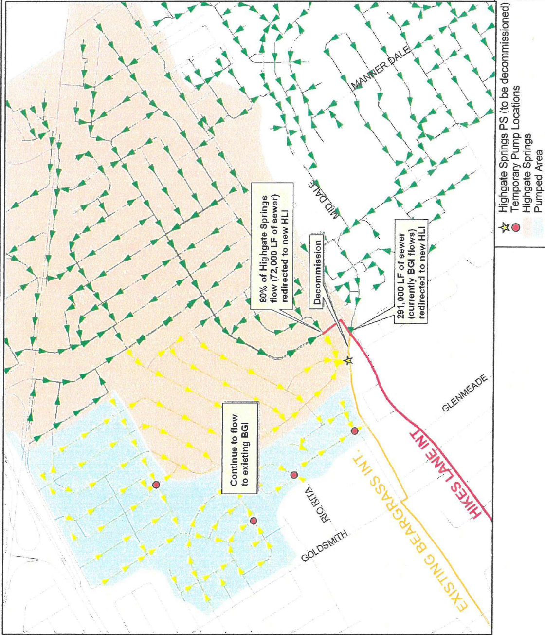
FIGURE 4 – CONVEYANCE OF FLOWS THROUGH HIKES POINT
