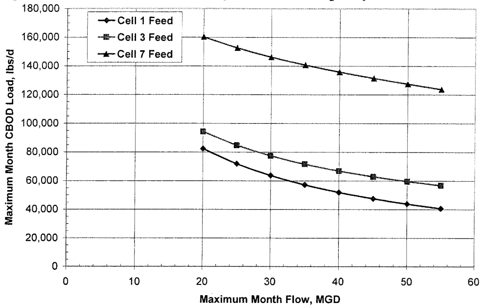
Figure 9: Wet Weather Secondary Treatment Capacity
