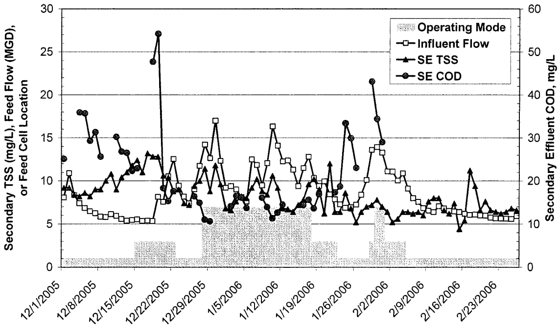
Figure 5: Aeration Basin 2 Wet Weather Performance
